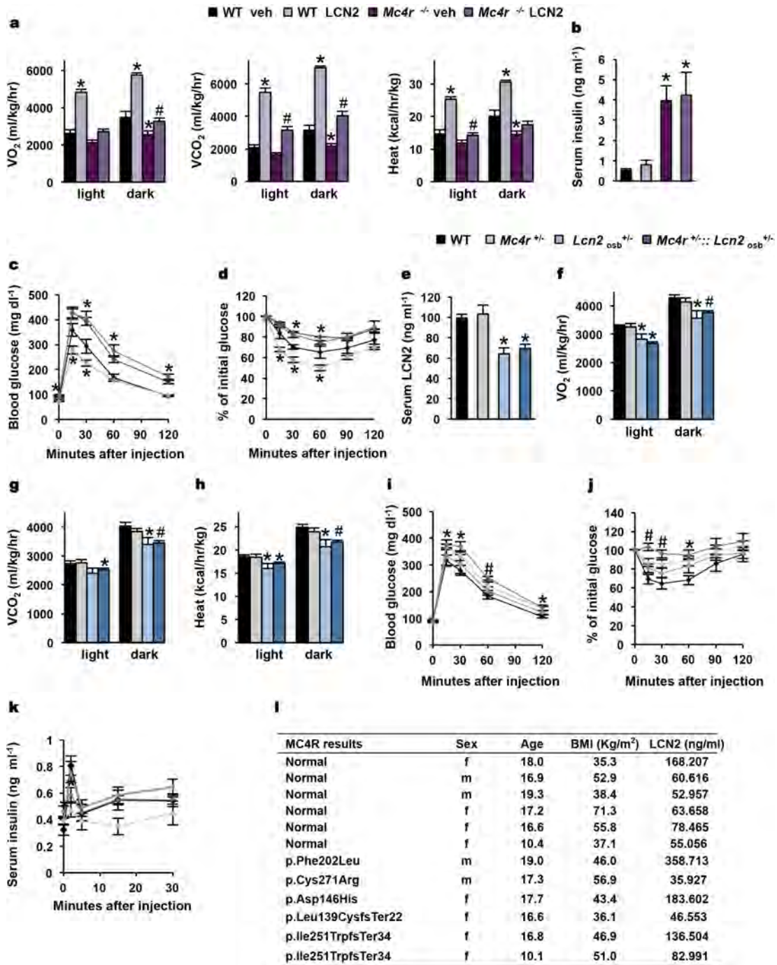
Extended Data Figure 10 | MC4R is required for the improvement in glucose metabolism and energy expenditure by LCN2. a–d, Mc4r -/- and wild-type littermates were treated with LCN2 (150 ng/g/day) or vehicle for 8 weeks. a, Indirect calorimetry measurements. b, Serum insulin levels. c, Glucose tolerance test. d, Insulin tolerance test. e–k, Serum levels of LCN2 (e), indirect calorimetry measurements (f–h), glucose tolerance test (i), insulin tolerance test (j) and glucose-stimulated insulin secretion (k) in Mc4r +/- , Lcn2 osb +/- , Mc4r +/- :: Lcn2 osb +/- and wild-type littermates. Data
