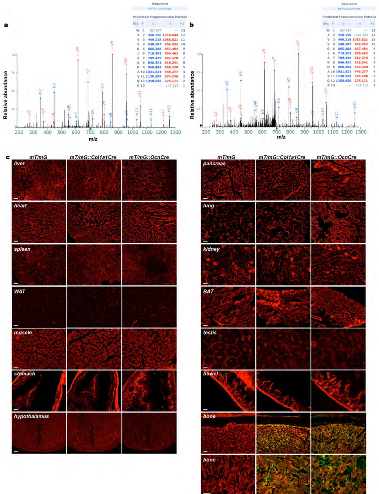
Extended Data Figure 2 | Osteoblast-specific activation of Cre in Col1a1-Cre and Bglap-Cre mice. a, b , Tandem mass spectrum of an eluted peptide fragment of bone-derived (a) and fat-derived (b) LCN2. c , Specific expression of Cre in osteoblasts, but not any other tissues in mT/mG::Col1a1-Cre mice and in mT/mG::Bglap-Cre mice. Scale bars, 100 \mu m. Results are representative of three independent experiments.
